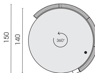
Element, round 360° rotational function parasol fixture right 761DF*
